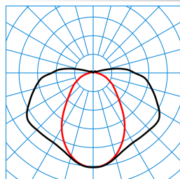
Acquex LED-M 0.6 20-840 ET PC EB3 TX774464
