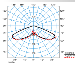
Publisca P1-RB6L/2400-740 3G1S ETDD (CLO initial value)
