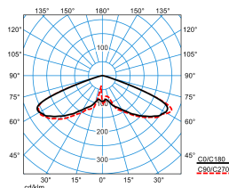
Publisca P1-RB6L/2400-740 3G1S ETDD (CLO end value)
