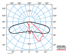
Publisca P1-AB2L/2400-740 3G1S ETDD (CLO initial value) TX301156 DIN 5040: A30 UTE: 1,00 l DLOR: 100 % ULOR: 0 % CEN Flux Code: 34 71 96 100 100
