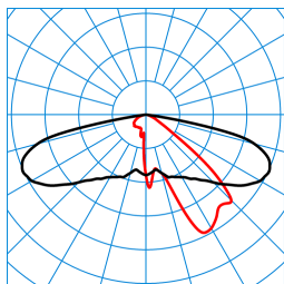
Publisca P1-AB2L/2400-740 3G1S ETDD (CLO initial value) TX301156 ■ C0 - C180 ■ C90 - C270 DIN 5040: A30 UTE: 1,00 l DLOR: 100 % ULOR: 0 % CEN Flux Code: 34 71 96 100 100
