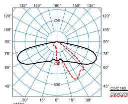
Publisca P1-AB2L/2400-740 3G1S ETDD (CLO end value) TX301841 DIN 5040: A30 UTE: 1,00 l DLOR: 100 % ULOR: 0 % CEN Flux Code: 34 71 96 100 100
