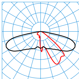
Publisca P1-AB2L/2400-740 3G1S ETDD (CLO end value) TX301841 ■ C0 - C180 ■ C90 - C270 DIN 5040: A30 UTE: 1,00 l DLOR: 100 % ULOR: 0 % CEN Flux Code: 34 71 96 100 100
