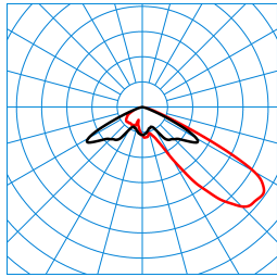
LnPlus 70-AM19L/42000-740 56G1 ETDD (CLO initial value) TX377444 ■ C0 - C180 ■ C90 - C270 DIN 5040: A30 UTE: 1,00 J DLOR: 100 % ULOR: 0 % CEN Flux Code: 26 78 99 100 100
