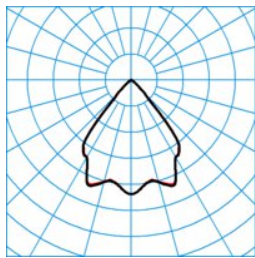
ELINE HE CLW1940 830 L150 1 20 ■ C0 - C180
