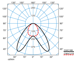
LPNT 3P2 L-DAW 80-940 M72 ETBLE 05
