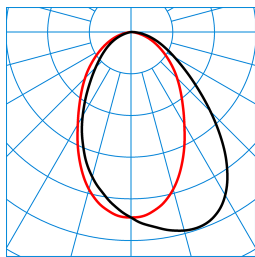
ArimoFit G2 Act M57 D-WW 42-8 ETDD8 (ActDSU) TX376396 ■ C0 - C180 ■ C90 - C270 DIN 5040: A50 UTE: 1,00 C DLOR: 100 % ULOR: 0 % CEN Flux Code: 61 87 98 100 100 0 0 0 0
