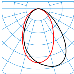
ArimoFit G2 Act M57 D-WW 42-8 ETDD8 (ActDWW) TX376390 ■ C0 - C180 ■ C90 - C270 DIN 5040: A50 UTE: 1,00 C DLOR: 100 % ULOR: 0 % CEN Flux Code: 61 87 98 100 100 0 0 0 0
