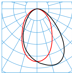
ArimoFit G2 Act M57 D-WW 42-8 ETDD8 (ActDCW) TX376383 ■ C0 - C180 ■ C90 - C270 DIN 5040: A50 UTE: 1,00 C DLOR: 100 % ULOR: 0 % CEN Flux Code: 61 87 98 100 100 0 0 0 0
