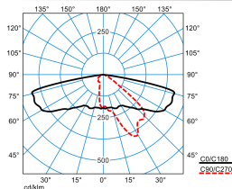
9301K AB2L-SLR2/3200-740 4G3 ET(CLO initial value)
