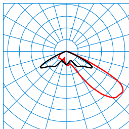
LnPlus 70-AM19L/68000-730 56G1 ETDD (CLO initial value) TX390184 ■ C0 - C180 ■ C90 - C270 DIN 5040: A30 UTE: 1,00 J DLOR: 100 % ULOR: 0 % CEN Flux Code: 26 78 99 100 100
