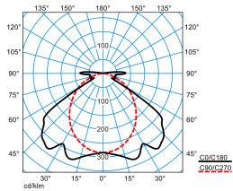
Nextrema G3 B 40-840 ET +HFS LV TWP PC TX768166
