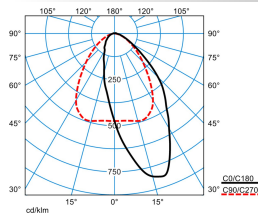
ELINE HE LAN100 865 L225 1 20
