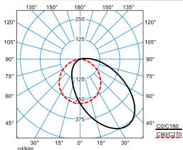
Sanesca W2 LED2600-840 03 (reading light)
