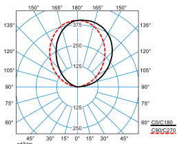
Sanesca W2 LED2600-840 03
