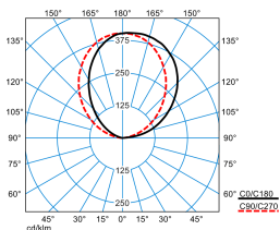
Sanesca W2 LED2600-840 03 (room light)
