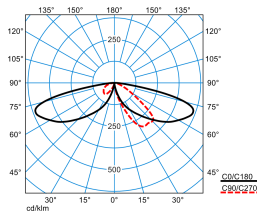
LTX KT-AB2L-LRA/2600-730 3G1 ETDD
