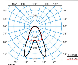
ELINE LDAN40-110 ML 830 L150 0 20
