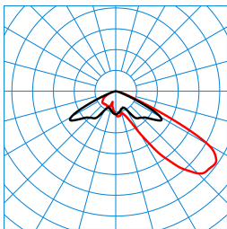
LnPlus 70-AM19L/42000-722 56G1 ETDD (CLO initial value) TX377348 ■ C0 - C180 ■ C90 - C270 DIN 5040: A30 UTE: 1,00 J DLOR: 100 % ULOR: 0 % CEN Flux Code: 26 78 99 100 100
