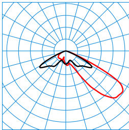
LnPlus 70-AM19L/42000-722 56G1 ETDD (CLO end value) TX377173 ■ C0 - C180 ■ C90 - C270 DIN 5040: A30 UTE: 1,00 J DLOR: 100 % ULOR: 0 % CEN Flux Code: 26 78 99 100 100
