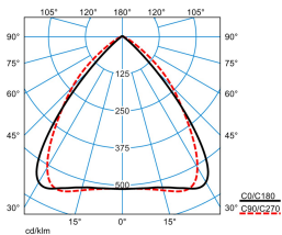
ELINE LN40-110 ML 865 L150 0 50
