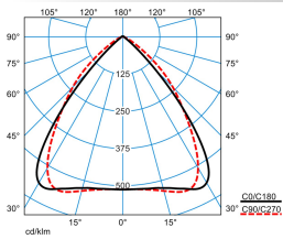
ELINE LN40-110 ML 865 L150 0 50
