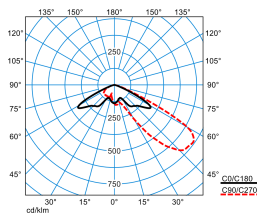
LnPlus 40-AM19L/3200-722 4G1 ETDD (CLO initial value) TX377689
