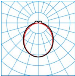
ELINE HE+ DSL100 840 L225 1 20 ■ C0 - C180
