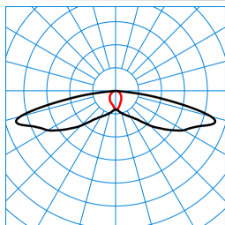
LIQ 50N-SB3L-LRA/1000-740 2G1 ETDD (CLO end value) TX779808
