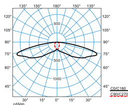
LIQ 50N-SB3L-LRA/1000-740 2G1 ETDD (CLO initial value) TX779813
