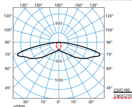
LIQ 50N-SB3L-LRA/1000-740 2G1 ETDD (CLO end value) TX779808
