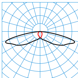
LIQ 50N-SB3L-LRA/1000-740 2G1 ETDD (CLO initial value) TX779813
