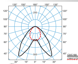
ELINE LDAW100 865 L225 1 20
