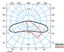
LIQ 50N-AB2L-LRA/4200-740 6G1 ETDD (CLO initial value) TX779079
