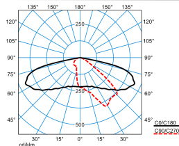
LIQ 50N-AB2L-LRA/4200-740 6G1 ETDD (CLO end value) TX779073
