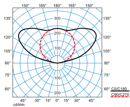
E-Line PRO 78ACT HE I-UW 15ETDD8 L75 01 Blank (ACTDWW)
