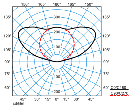
E-Line PRO 78ACT HE I-UW 15ETDD8 L75 01 01 (ACTDWW)
