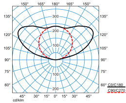
E-Line PRO 78ACT HE I-UW 15ETDD8 L75 03 Blank (ACTDWW)
