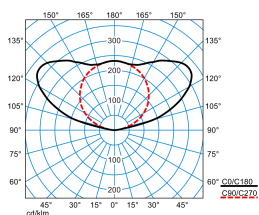
E-Line PRO 78ACT HE I-UW 15ETDD8 L75 05 05 (ACTDWW)
