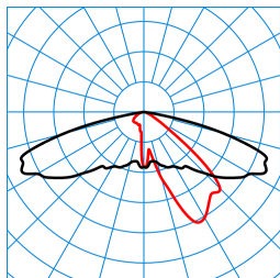
Publisca P1W-AB2L-LRA/3800-740 6G1S ET (CLO initial value) TX301774 ■ C0 - C180 ■ C90 - C270 DIN 5040: A30 UTE: 1,00 G DLOR: 100 % ULOR: 0 % CEN Flux Code: 34 72 97 100 100 0 0 0 0
