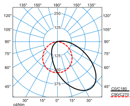
Sanesca W2 4600-8TW ETDD/ET 830 03 (DWW) (reading_light)
