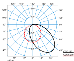
Sanesca W2 4600-8TW ETDD/ET 830 03 (DSU) (reading_light)
