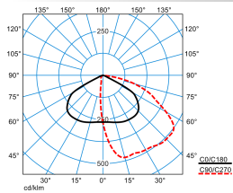
Inveria C 210 AM21R/3700-830 1G1P ETDD TX460581
