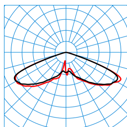
Publisca P2-RB6L-LR/2400-730 3G1S ET (CLO initial value) TX301745 ■ C0 - C180 ■ C90 - C270 DIN 5040: A20 UTE: 1,00 J DLOR: 100 % ULOR: 0 % CEN Flux Code: 20 57 98 100 100
