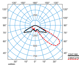
LnPlus 60-AM19L/20000-727 24G1 ETDD (CLO end value) TX377321
