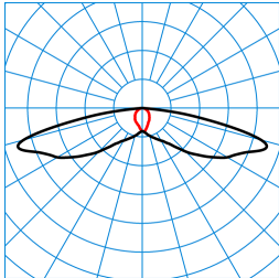
LIQ 50N-SB3L-LR/1350-722 2G1 ET (CLO end value) TX779596 ■ C0 - C180 ■ C90 - C270 DIN 5040: A30 UTE: 1,00 l DLOR: 100 % ULOR: 0 % CEN Flux Code: 31 64 92 100 100
