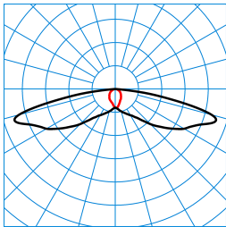
LIQ 50N-SB3L-LR/1350-722 2G1 ET (CLO initial value) TX779603 ■ C0 - C180 ■ C90 - C270 DIN 5040: A30 UTE: 1,00 l DLOR: 100 % ULOR: 0 % CEN Flux Code: 31 64 92 100 100
