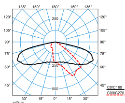
LIQ 50N-AB2L-LRA/135/165/20-740 2G1 ETDD (CLO initial value) TX778152
