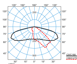
LIQ 50N-AB2L-LRA/135/165/20-740 2G1 ETDD (CLO end value)
