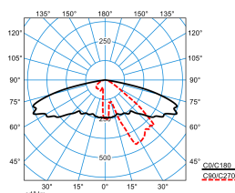
Publisca P1W-AB2L/1500-730 2G1S ETDD (CLO end value)
