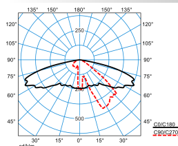
Publisca P1W-AB2L/1500-730 2G1S ETDD (CLO initial value)
