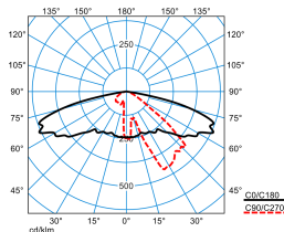
Publisca P1W-AB2L-LRA/1500-740 2G1S
