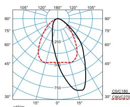
ELINE HE LAN60-160 ML 840 L225 2 20
