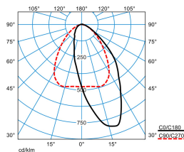
ELINE HE LAN60-160 ML 840 L225 4 20
