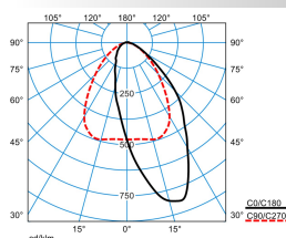
ELINE HE LAN60-160 ML 840 L225 0 20
