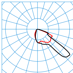
LIQ 50N-FR1L/4200-727 4G1 ET (CLO initial value) TX780578 ■ C0 - C180 ■ C90 - C270 DIN 5040: A40 UTE: 1,00 F DLOR: 100 % ULOR: 0 % CEN Flux Code: 41 83 99 100 100
