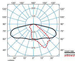
LIQ 50-AB2L-LR/1200-730 2G1S ET TX777282 DIN 5040: A30 UTE: 1,00 G DLOR: 100 % ULOR: 0 % CEN Flux Code: 36 71 96 100 100
