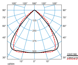
ELINE HE LW2240-120 ML 840 L150 0 50
