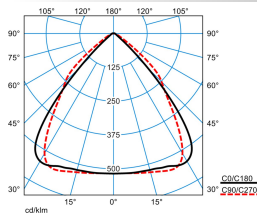
ELINE HE LW2240-120 ML 840 L150 0 50
