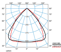
ELINE HE LW2240-120 ML 840 L150 2 50
