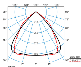
ELINE LW2240-110 ML 840 L150 4 20
