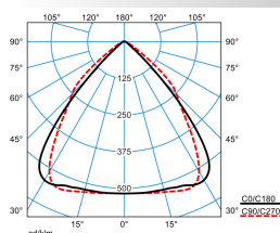
ELINE LW2240-110 ML 840 L150 0 20
