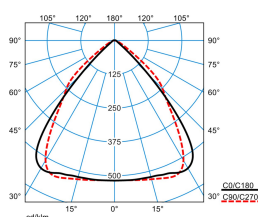
ELINE LW2240-110 ML 840 L150 2 20
