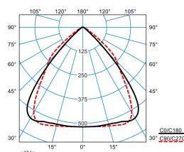
ELINE LW2240-110 ML 840 L150 4 20
