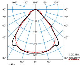
SFlow C3-L MRW LED4000-840 ETDD LLWS 01 TX771985
