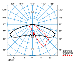
Publisca P2-AB2L/5600-740 6G1S ETDD (CLO initial value)
