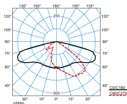
LIQ 70N-AB7L-LR-SLR2/16000-730 12G1 ET (CLO initial value) TX778044
