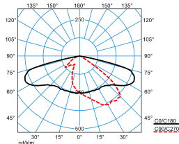
LIQ 70N-AB7L-LR-SLR2/16000-730 12G1 ET (CLO end value) TX778040
