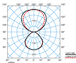
Luceos D/H1-L CDP 4000-8TW ETDD 03 (Pendant ZS/ZST) (CWW)
