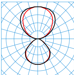
Luceos Act D/H1-L CDP 4000 ETDD 03 (Pendant ZS/ZST) (ActCCW) TX194575
