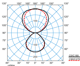
Luceos D/H1-L CDP 4000-8TW ETDD 03 (Pendant ZS/ZST) (CCW)
