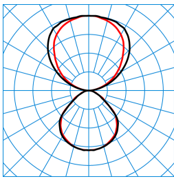
Luceos Act D/H1-L CDP 4000 ETDD 03 (Pendant ZS/ZST) (ActCWW) TX194577
