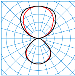
Luceos Act D/H1-L CDP 4000 ETDD 03 (Pendant ZS/ZST) (ActCSU) TX194576
