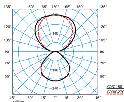
Luceos D/H1-L CDP 4000-8TW ETDD 03 (Pendant ZS/ZST) (CSU)
