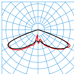
Publisca P2-RB6L-LR/2400-740 3G1S ET (CLO initial value) TX300674 ■ C0 - C180 ■ C90 - C270 DIN 5040: A20 UTE: 1,00 J DLOR: 100 % ULOR: 0 % CEN Flux Code: 20 57 98 100 100
