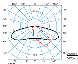
LIQ 50N-AB2L-LRA/3800-730 4G1 ETDD (CLO end value)
