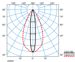
Altigo G2 90 SE6L/3000-830 1G1P + VE IP66 24V DC 60W TX120422
