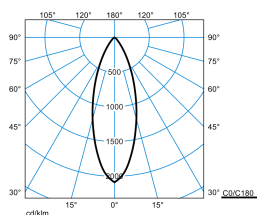
Amatris RC2 SRRFL 12-9MC ETD-PD 05 + HC-19 05 (stage 2)
