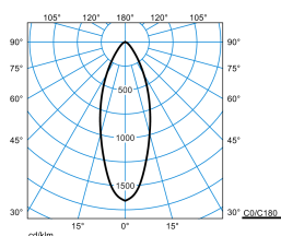
Amatris RC2 SRRFL 12-9MC ETD-PD 05 + PC IP54 (stage 3)
