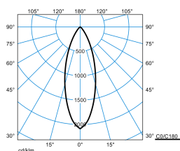
Amatris RC2 SRRFL 12-9MC ETD-PD 05 + HC-19 05 (stage 3)
