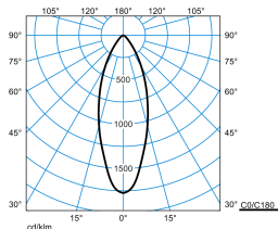
Amatris RC2 SRRFL 12-9MC ET-PD 05 (stage 3)
