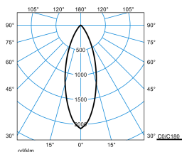
Amatris RC2 SRRFL 12-9MC ETD-PD 05 + HC-19 05 (stage 1)
