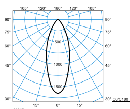
Amatris RC2 SRRFL 12-9MC ETD-PD 05 + PC IP54 (stage 2)
