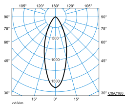
Amatris RC2 SRRFL 12-9MC ETD-PD 05 + PC IP54 (stage 1)
