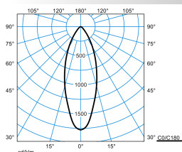
Amatris RC2 SRRFL 12-9MC ET-PD 05 (stage 1)
