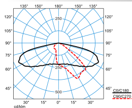
LIQ 50N-AB2L-LR/220/260/320-722 4G1 ET (CLO initial value)
