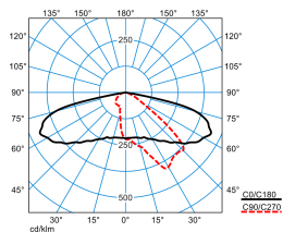
LIQ 50N-AB2L-LR/220/260/320-722 4G1 ET (CLO end value)
