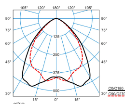
ELINE HE LW60-160 ML 840 L225 4 50
