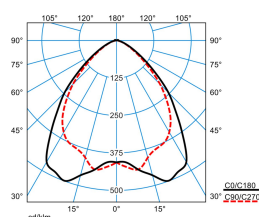
ELINE HE LW60-160 ML 840 L225 2 50
