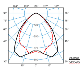
ELINE HE LW60-160 ML 840 L225 0 50
