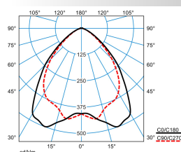
ELINE HE LW60-160 ML 840 L225 0 50
