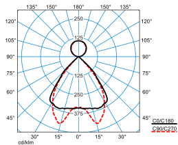
SFlow H2-L MRX LED6400-830 ET 01 TX721235
