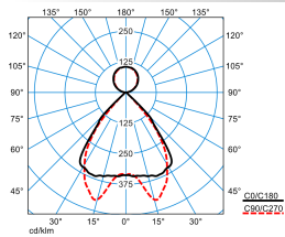
SFlow H2-L MRX LED6400-830 ET 01 TX770387
