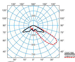
LnPlus 40-AM19L/2200-740 2G1 ETDD (CLO initial value) TX377253
