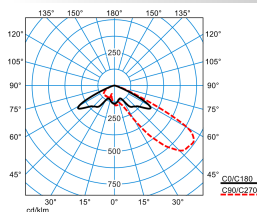
LnPlus 40-AM19L/2200-740 2G1 ETDD (CLO end value) TX377033
