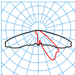
Publisca P1W-AB2L-LR/3800-730 6G1S ET (CLO initial value) TX301309 ■ C0 - C180 ■ C90 - C270 DIN 5040: A30 UTE: 1,00 G DLOR: 100 % ULOR: 0 % CEN Flux Code: 34 72 97 100 100 0 0 0 0
