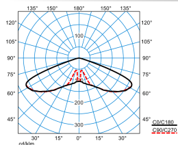
Publisca P2-RB6L-LR/1000-740 2G1S
